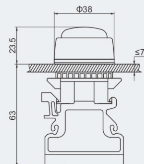
Cover mounting
