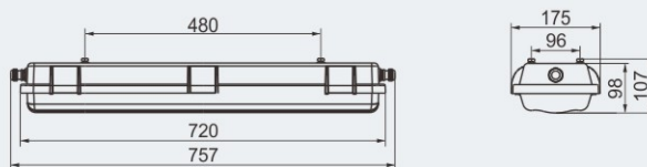
Type I: BnY81-LED 9 x 2□; BnY81-LED 9 x 2□J; BnY81-LED 14 x 2□; BnY81-LED 14 x 2□J; BnY81-LED 20□; BnY81-LED 20□J; BnY81-LED 40□
