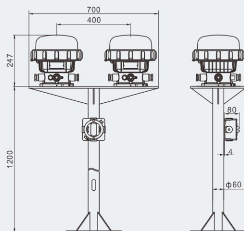
Drawings of main (spare) caution spotlight fittings
