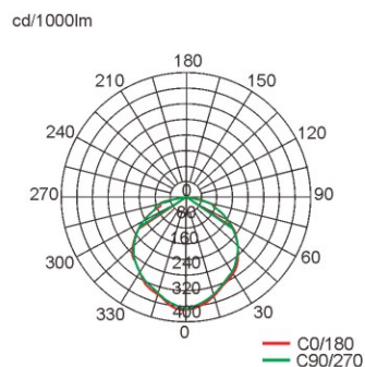
配光曲线 Light distribution curve
