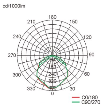
配光曲线 Light distribution curve
