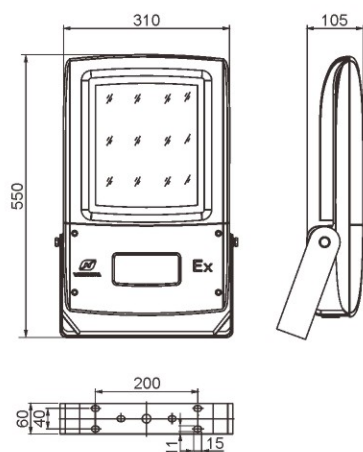
50W, 70W, 100W, 120W, 160W, 200W
